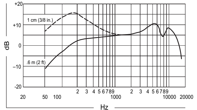
TYPICAL FREQUENCY RESPONSE FIGURE 1
